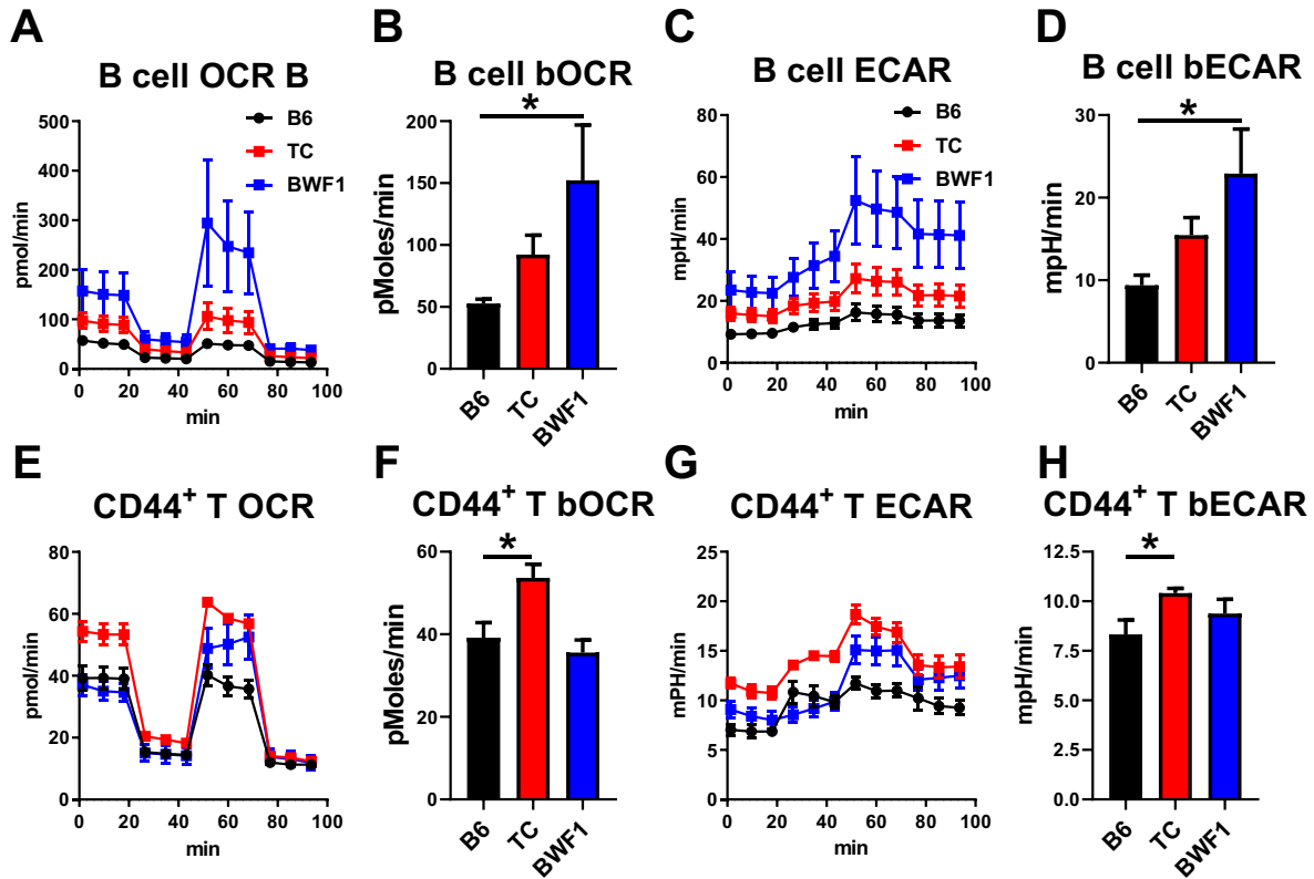
Supplemental figure 1. Mitochondrial stress test comparing B cells (A – D) and CD44 + CD4 + T cells between 2 month old B6 TC and BWF1 mice (N = 3 each). OCR time course (A and E) and basal OCR (B and F); ECAR time course (C and G) and basal ECAR (D and H). Mean \pm SEM, compared with one-tailed t tests, * P < 0.05.
